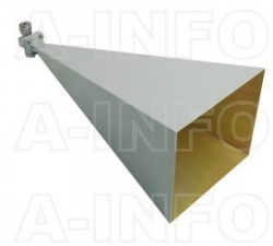
LB-75-25-C-7 Standard Gain Horn Antenna 10-15GHz 25dB Gain 7mm
