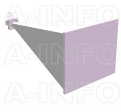
LB-75-25-C-7SPO Standard Gain Horn Antenna 10-15GHz 25dB Gain 7mm
