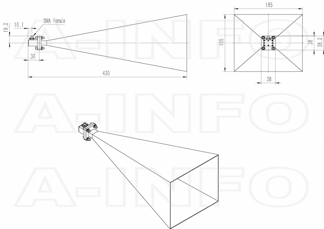
SMA-Female Output (P/N: LB-75-25-C-SF)
